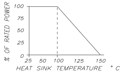
DERATING CURVE:
